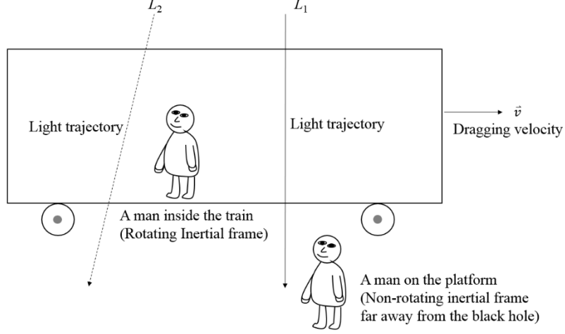
Figure 1. The observations of the light trajectory from different inertial frame. The rotating inertial frame has the tangential velocity v with respect to the Kerr-Newman black hole as the transparent train. An observer stays with the train and the other one is at rest on the platform. A light beam observed by the observer on the platform is perpendicular to the movement of the train as the light trajectory L_1 . The same light beam observed by the observer moving with the train is the light trajectory L_2 .
