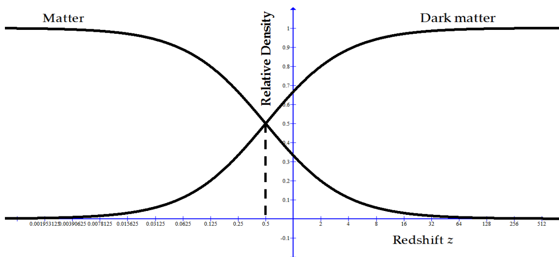
Figure 5. Relative matter and dark matter (and their relative energies) densities as a function of redshift z .
