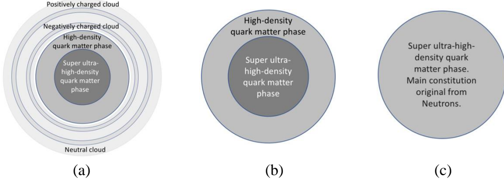
Fig. 1 (a) The nucleus of the black hole is mainly consisting of materials the from high-density the quark matter phase to super ultra-high-density quark matter phase. It is surrounded by small negatively and positively charged particles as well as neutral ones to form a structure like a very big atom. The totally charges Q are fluctuated in time. (b) The nucleus of the black hole still contains materials from high-density quark matter phase to super ultra-high-density quark matter phase. Its total charges Q is fluctuation in time. (c) The nucleus of the black hole is mainly consisting of neutrons from high-density quark matter phase to super ultra-high-density quark matter phase to form a basic structure. The total charges Q are fluctuated in time.
