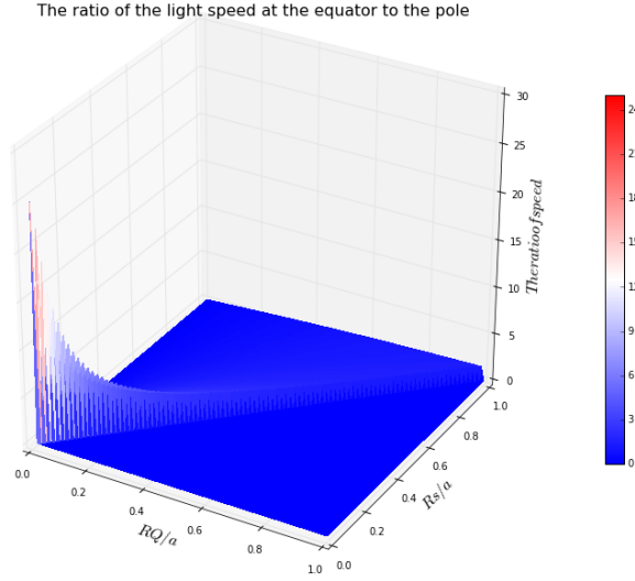
Fig. 2 The ration of the absolute speed of light at the equator to the pole at r=R_S . It is the function of R_Q/a and R_S/a and both ranges are between 0.01 to 1.00 with interval 0.01. The ratio of the light speed is as large as 25 times when a \gg R_Q and a \gg R_S in our calculations.
