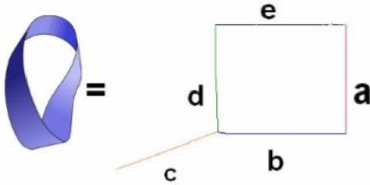
Figure 3 – Möbius equals a,b,c,d,e array
