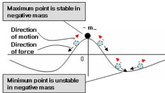
Figure 2: When there is negative mass in potential which has a point of maximum value and a point of minimum value.
