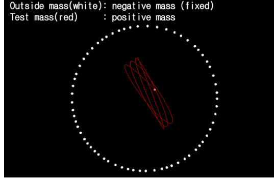
Figure 6: White : negative mass(fixed), Red : positive mass(free). The positive mass vibrates.
