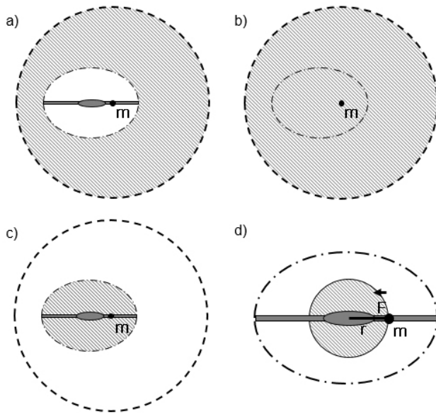
Figure 5: The structure of the galaxy surrounded by negative mass that is distributed equally.(a) The white area is the area where negative mass almost does not exist.
