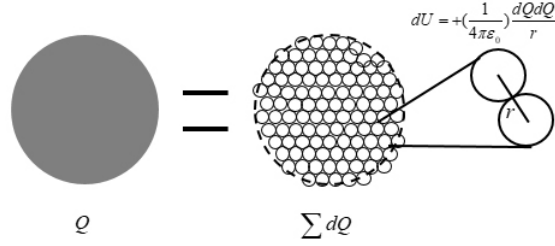
Figure 4: Since all charge Q is a set of infinitesimal charge dQ s and each dQ is electromagnetic source, too, there exists electrostatic potential energy among each of dQ s.
