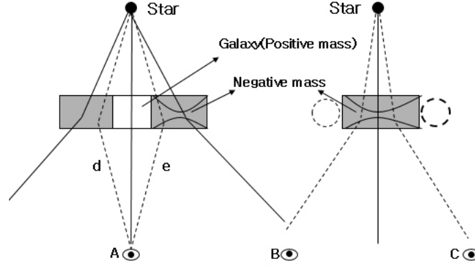
Figure 6: Concave Gravitational lensing effect. The left side is the Gravitational lensing effect that occurs when the galaxy is surrounded by negative mass. The right side is Gravitational lensing effect that occurs when negative mass exists alone
