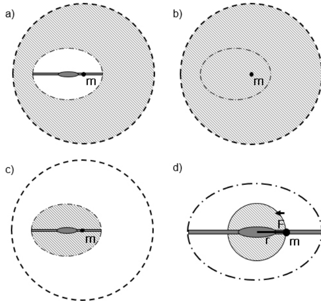
Figure 4: The structure of the galaxy surrounded by negative mass that is distributed equally.(a) The white area is the area where negative mass almost does not exist. The oblique line area is the area where negative mass is distributed.
