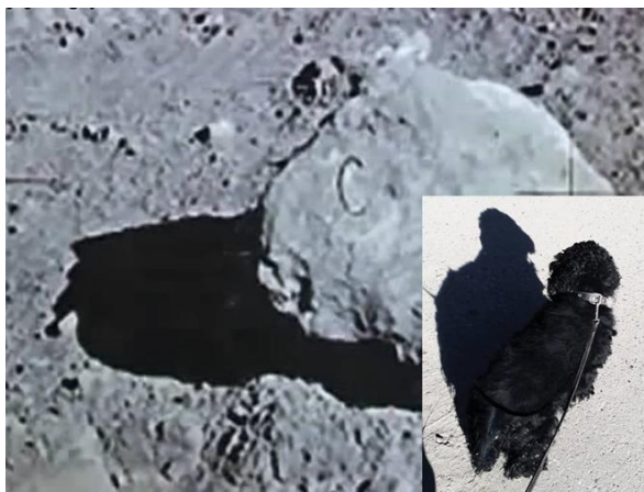
Fig. 1. Shadows from objects on the Moon and on Earth
