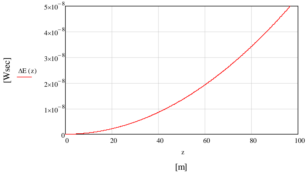
FIG.1 the dependency of energy loss due to radiation for a 10,000kg test body free falling in a uniform gravitational field equal to Earth’s gravity on the travelled distance z of the fall.
