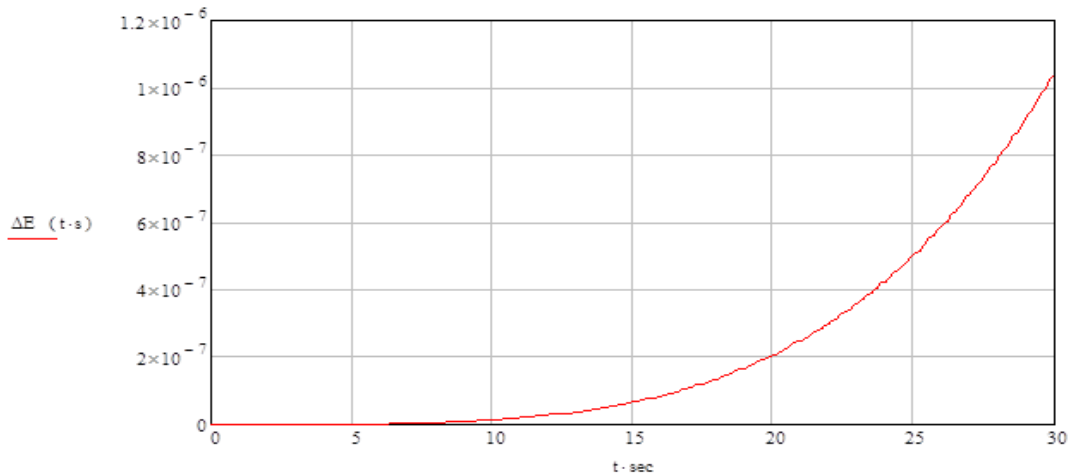
FIG.1 the dependency of energy loss due to radiation for a 100kg test body free falling in a uniform gravitational field equal to Earth's gravity. The loss for a 30 sec fall is about 1.0 micro Joules.
