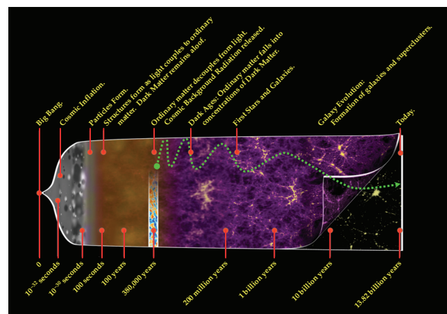
Fig. 2 Condom Cosmology: Starting from a point of infinite density the Universe is commonly supposed to have, in the first 10^{-32} seconds, blown up by the primordial “inflaton field.” Supposedly, the rest is history.
