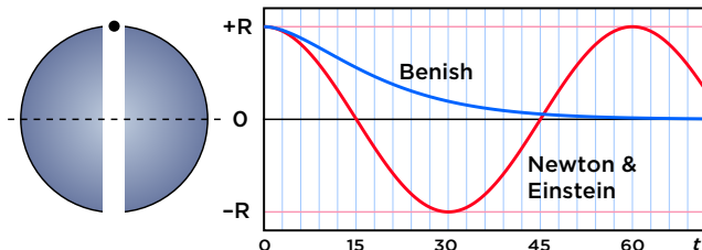
Fig. 3 Schematic showing competing predictions: Simple harmonic motion (red curve) vs. asymptotic approach to the center. The 60-minute oscillation period corresponds to a spherical source mass made of lead.
