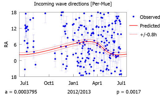
Fig. 10: Points show the RAs of the 198 incoming wave directions. The red curve shows RA values obtained from Eqn. (7) using our estimate of v_{WG} with RA = 4.50 h , dec = -80.6^0 and speed = 504 km/s . Of 198 points, 25 lie within \pm 0.8 RA hours of this curve. The probability of this degree of closeness arising from chance is P_{RA} = 0.0017 .
