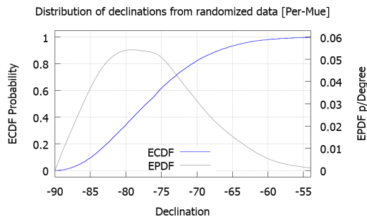
Fig. 12: Blue curve shows empirical cumulative distribution function for declinations derived from randomized travel times. That is, for each RA of each day to be simulated, a travel time was selected at random from the set of 24 \times 198 travel times that had been determined for the 198 days that had complete data. Gray curve shows the corresponding empirical probability distribution function.
