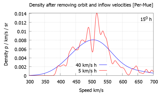
Fig. 8: Probability density plots of galactic wave speed for waves with galactic directions approximately parallel to our best estimate of the direction of \mathbf{v}_{WG} . The angular bandwidth of 15^\circ is centered on \mathbf{v}_{WG} and gives greater weight to speeds of waves with directions closer to \mathbf{v}_{WG} .
