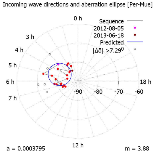
Fig. 11: Points show the 25 incoming wave directions whose RAs in Fig. 10 are within \pm 0.8 h of predicted RA. The blue orbital aberration ellipse shows variation of predicted RA and declination during a year due to the combined effect of Earth orbital and Earth and Sun inflow velocities. Of the 25 points, 20 shown as solid have declinations that lie within \pm 7.29^\circ of predicted values. The probability of this closeness being a result of chance is P_{dec} = 2.9 \times 10^{-4} .
