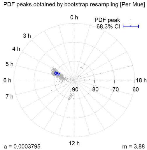
Fig. 9: Example of 2000 iterations of bootstrap resampling. Each point shows a peak of probability density calculated from a different set of 198 wave directions randomly selected from the 198 available directions.
