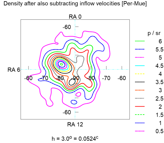
Fig. 7: Probability density after removing Earth orbital and Sun and Earth inflow velocities.
