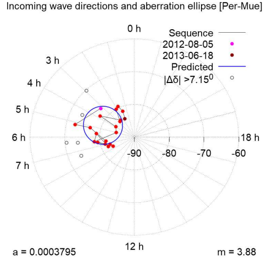
Fig. 10: Points show the 25 incoming wave directions whose RAs in Fig. 9 are within \pm 0.8 h of predicted RA. The blue orbital aberration ellipse shows variation of predicted RA and declination during a year due to the combined effect of Earth orbital and Earth and Sun inflow velocities. Of the 25 points, the 20 shown as solid have declinations that lie within \pm 7.15^\circ of predicted values. The probability of this closeness being a result of chance is P_{dec} = 0.00015 .
