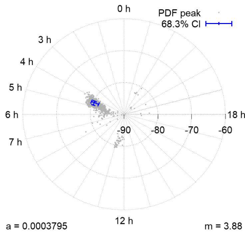
PDF peaks obtained by bootstrap resampling [Per-Mue]
