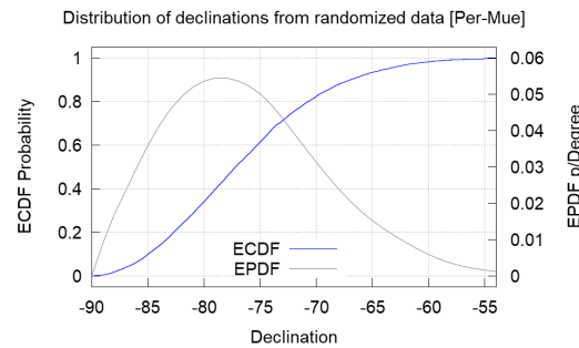
Fig. 11: Blue curve shows empirical cumulative distribution function for declinations derived from randomized travel times. That is, for each RA of each day to be simulated, a travel time was selected at random from the set of 24 \times 198 travel times that had been determined for the 198 days that had complete data.
