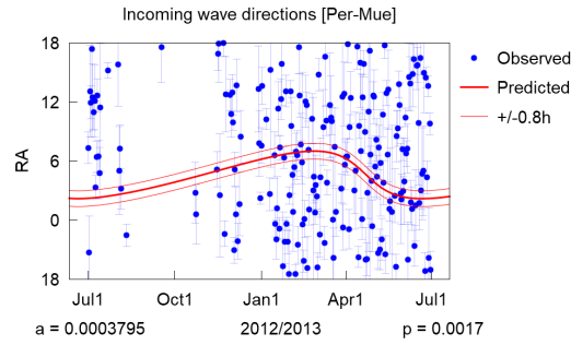
Fig. 9: Points show the RAs of the 198 incoming wave directions. The red curve shows RA values obtained from Eqn. (7) using our estimate of \mathbf{v}_{WG} with RA = 4.49 h , dec = -80.4^0 and speed = 508 km/s . Of 198 points, 25 lie within \pm 0.8 RA hours of this curve. The probability of this degree of closeness arising from chance is P_{RA} = 0.0017 .
