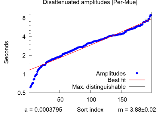
Fig. 4: Disattenuated amplitudes obtained from Perth-Muenster travel times by sorting the original values and then multiplying by a suitable value m to allow the best fit exponential curve to match the range of the detection process. Here use of a logarithmic vertical axis results in a straight line plot.
