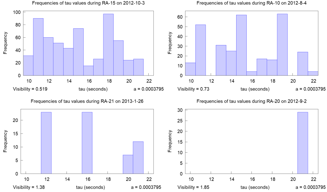
Fig. 2: Histograms of Perth-Manchester \tau values detected during different RA hours illustrating a range of signal visibilities from low to high. The multiple peaks are consistent with passage of non-distinguishable waveforms, w_n, w_{n+1}, w_{n+2} \dots etc. three to five seconds apart. Then the correlation of w_n at one detector with say w_{n+1} or w_{n+2} at the other, may be as large as the correlation with w_n . The single peak in the last histogram is consistent with passage of distinguishable waveforms.
