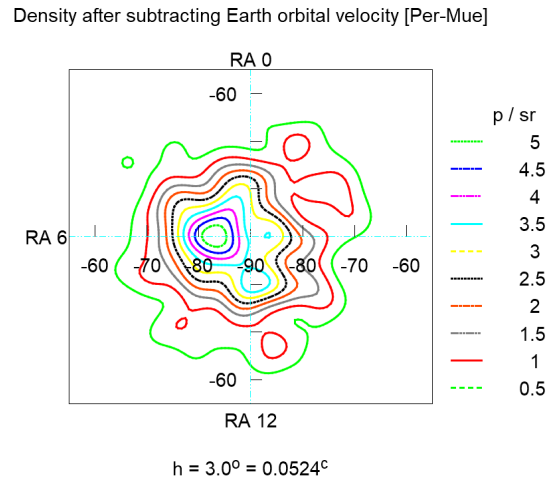
Fig. 6: Probability density after removing Earth orbital velocity.
