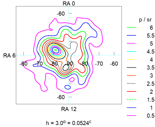
Fig. 7: Probability density after removing Earth orbital and Sun and Earth inflow velocities.
