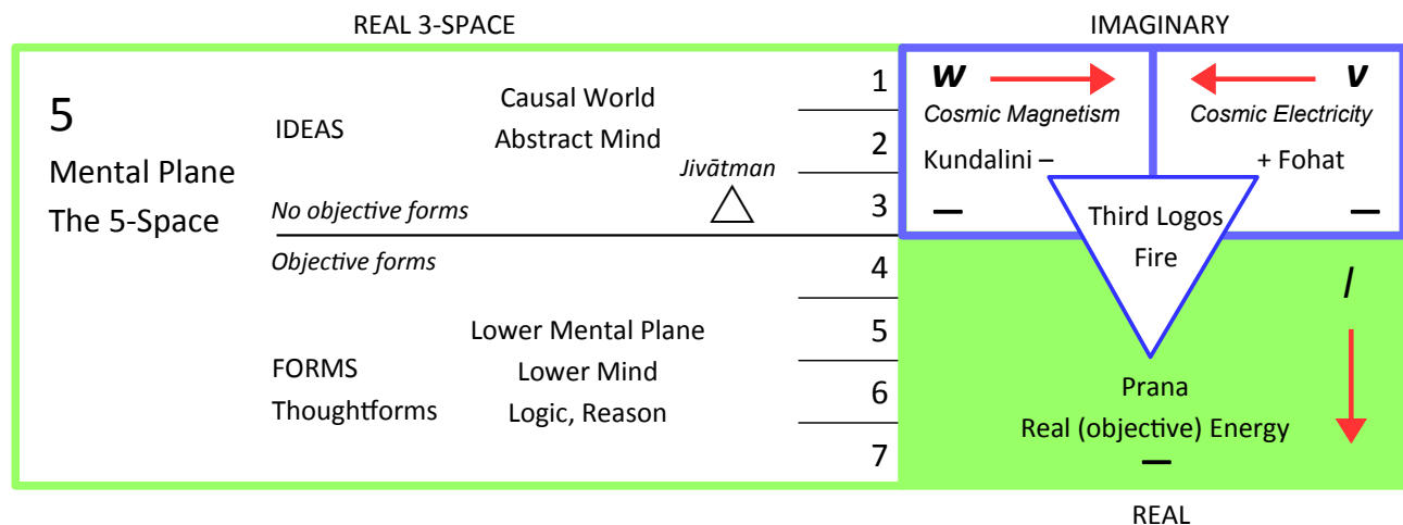
Figure 15: From Subjective to Objective
