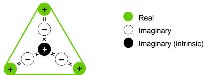
Figure 8: Imaginary Foundations of Real 3-Space
