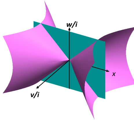
Figure 4: Null Surfaces in Minkowski 5-Space
