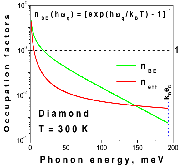
FIG. 3 (color online). The room-temperature spectral dependencies of the ‘standard’ Bose-Einstein occupation factor n_{\text{BE}}(\hbar\omega_q) and its ‘effective’ counterpart n_{\text{eff}}(\hbar\omega_q) , defined by Eq.(13). Both dependencies are evaluated for ground single-particle states of Debye acoustic phonons of the diamond with its Debye energy of k_B\theta_D = 193.0 meV ( \theta_D = 2240 K), indicated in the figure with the vertical dashed line. See further details in the main text.
