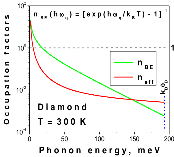
FIG. 3 (color online). The room-temperature spectral dependencies of the ‘standard’ Bose-Einstein occupation factor n_{\text{BE}}(\hbar\omega_q) and its ‘effective’ counterpart n_{\text{eff}}(\hbar\omega_q) , defined by Eq.(13). Both dependencies are evaluated for ground single-particle states of Debye acoustic phonons of the diamond with its Debye energy of k_B\theta_D = 193.0 meV ( \theta_D = 2240 K), indicated in the figure with the vertical dashed line. See further details in the main text.
