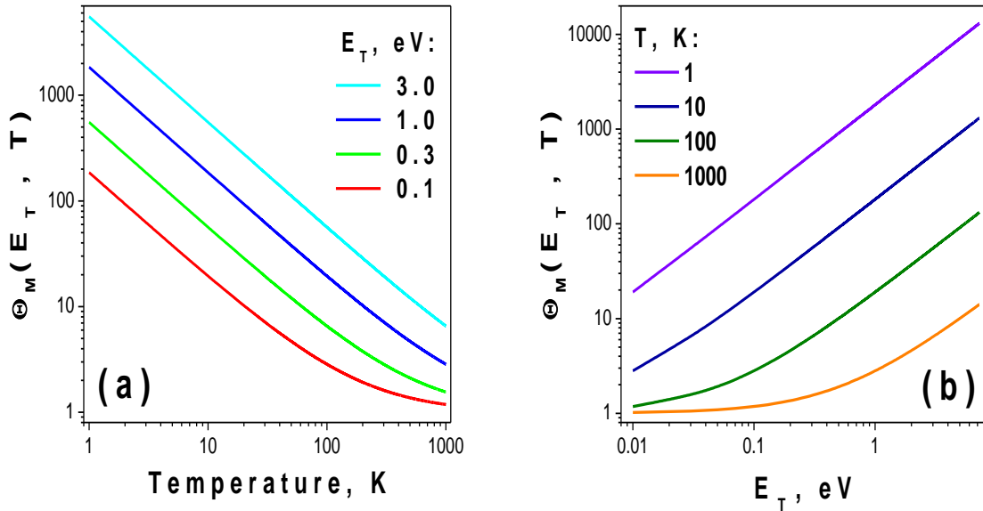
FIG. 2 (a), (b) (color online). Effects of (a) the absolute temperature T and (b) aggregate energy E_T of the phonon ensemble on the \Theta_M(E_T, T) function, defined by Eq.(7). The plotted curves are obtained via replacement of the \text{Int} function in this equation with its rational argument. Mind double-logarithmic scale(s) for both panels of the figure.
