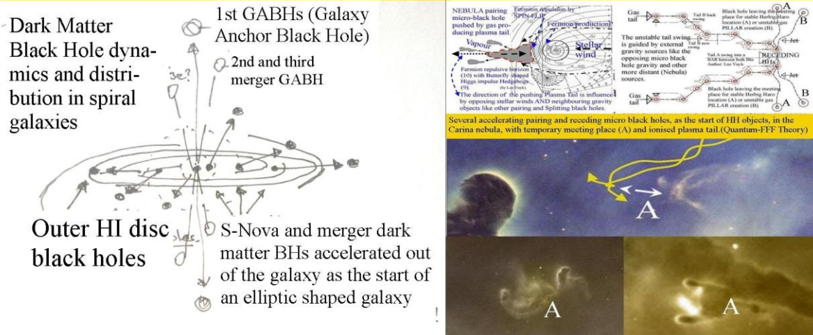
Figure, 28 . Dark Matter Black Hole dynamics in spiral galaxies.
