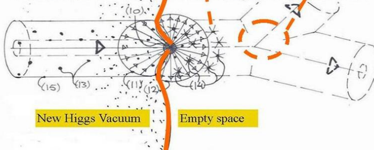
Figure 15, BBBH , the Big Bang Black Hole splintering into smaller BHs and evaporating into the oscillating Axion Higgs Vacuum lattice .
