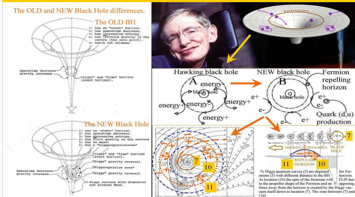
Figure 29, The new black hole
