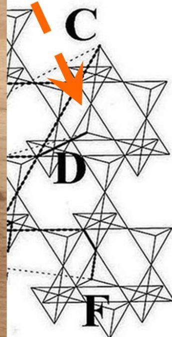
Figure 8, A stable black hole nucleus is large enough to “eat” the vacuum particles and grow by it.
