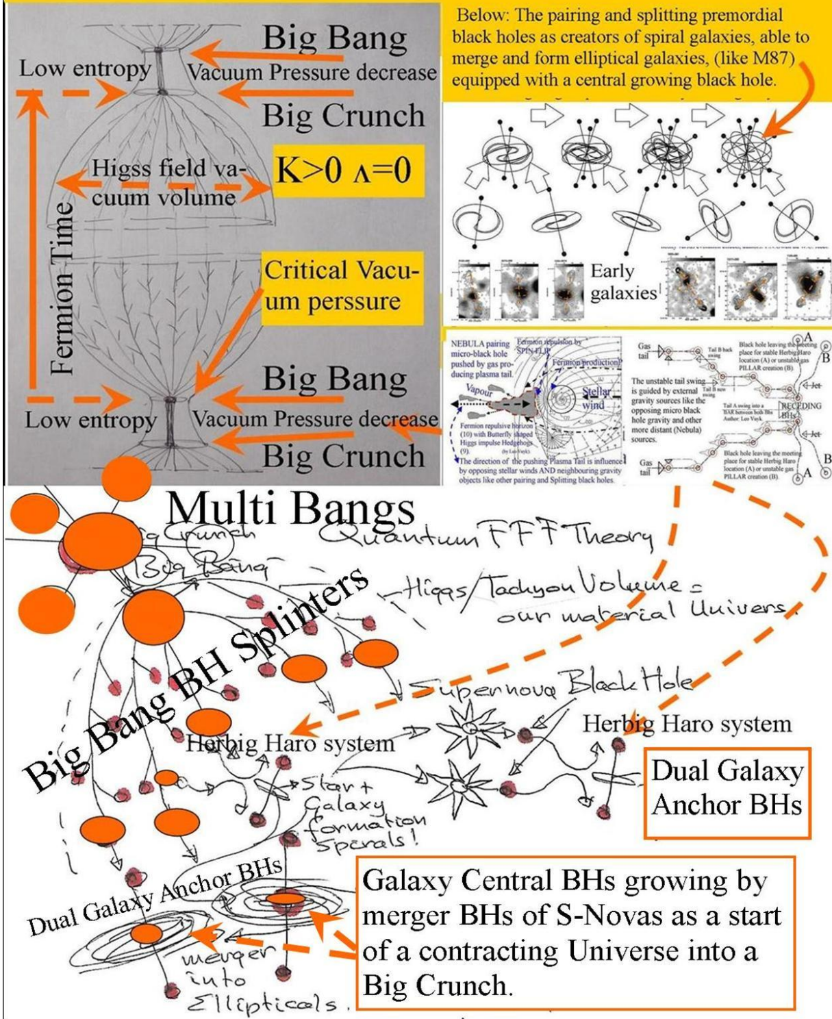
Figure 17, The Cyclic Multiverse.
