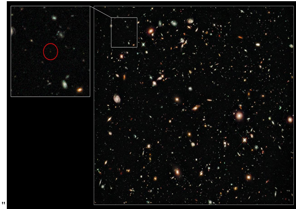
Fig. 1. Galaxies on the border of the universe
