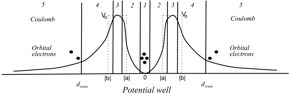
Figure 6: Potential well of an atom.
