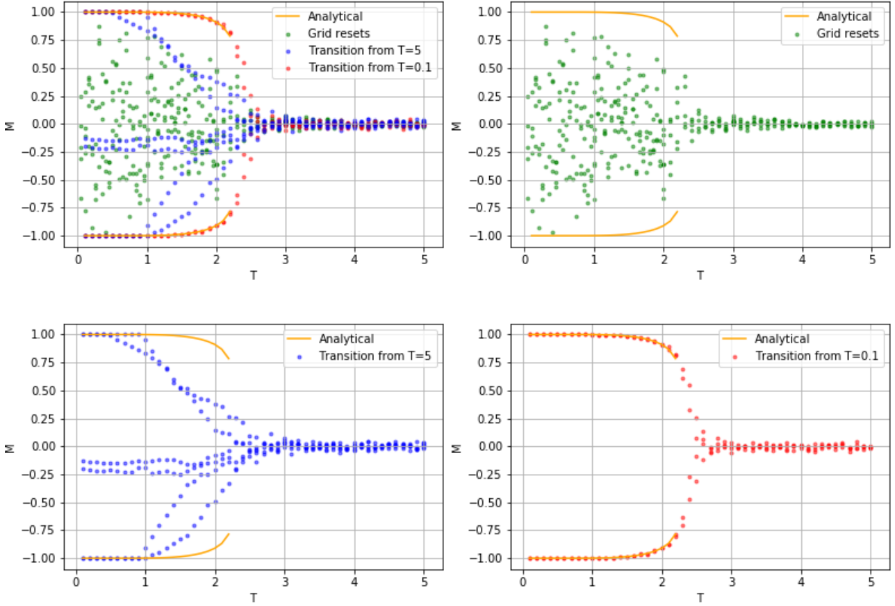
Figure 5: Plots of the average magnetization of spins as a function of temperature. The orange lines denote the value obtained through equation ??.
