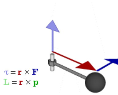
Figure 7: Torque and angular momentum vectors
