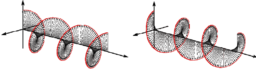
Figure 8: Left- and right-handed matter-wave
