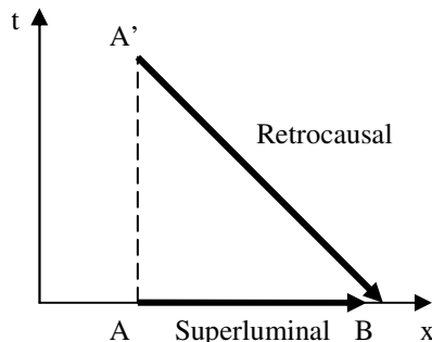
Figure 2a – Superluminal or Retrocausal?
