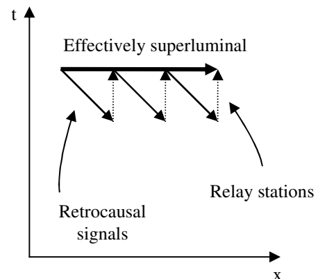
Figure 3 – A de-facto superluminal signal from a retrocausal signal
