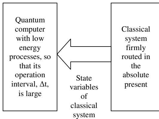
Figure 4 – “Quantum Clairvoyance” or just a State Predictor?
