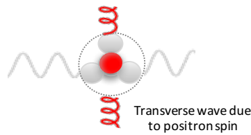
Fig 2.2.4 – Proton’s spin (anti-quark/positron spin in the center)
