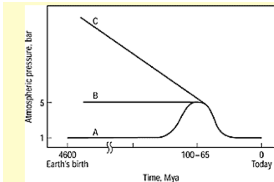
Figure 1. Three possible alternatives for the atmospheric pressure early in Earth's lifetime, given that it was at ~5 bar, ~100 Mya.
