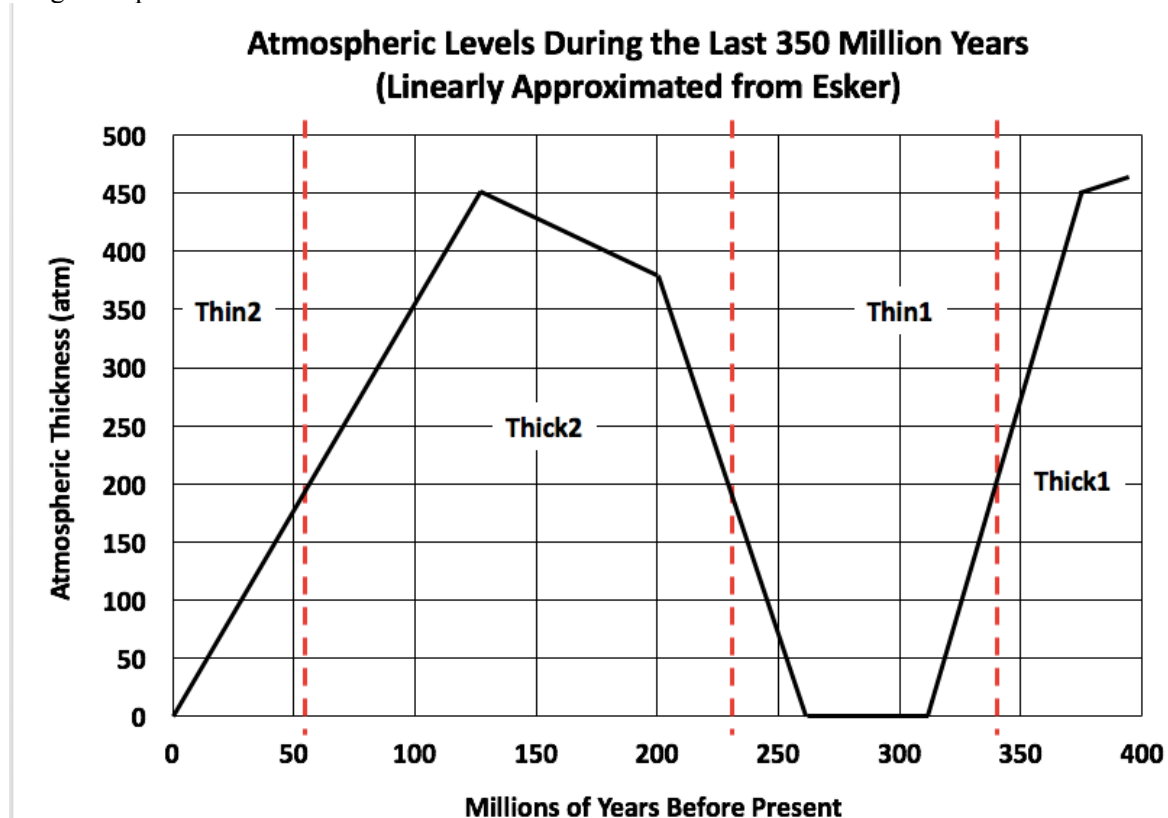
Figure 2. Atmospheric Levels during the Last 350 Million Years with Assumed Transition Times
