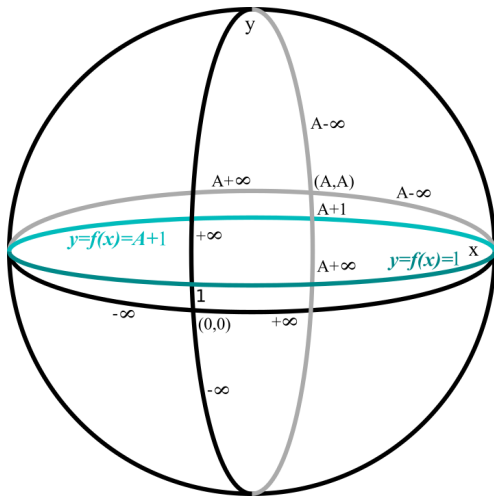
Figure 2: Graph of y = 1 and y = A + 1 .
