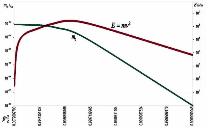
Figure 1. The varying laws of the static mass and energy of electron following its relative speed
