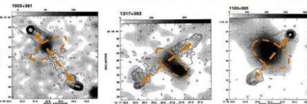
TWO pairing and receding micro black holes, propelled by unstable ionised gas tails, as observed in many Nebula: Carina, Eagle, Crab etc. creating HH objects or Gas Pillars.
