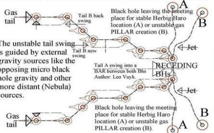
TWO pairing and receding micro black holes, propelled by unstable ionised gas tails, as observed in many Nebula: Carina, Eagle, Crab etc. creating HH objects or Gas Pillars.
