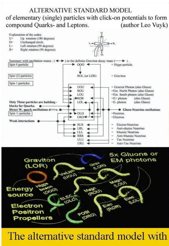
Figure 8, the alternative standard model ref. [5]
