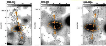
All images are copies from: The Astronomical Journal Vol 109 nr 2 Febr. 1995. the article is called: Faint B3 Radio Galaxies: Luminosity versus evolution effects, authors: F.N.Owen ad W.C. Keel.
