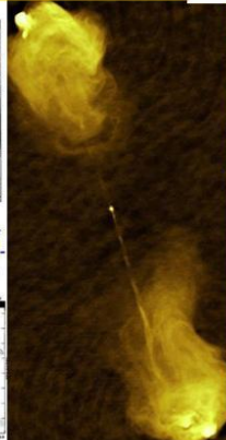
All images are copies from: The Astronomical Journal Vol 109 nr 2 Febr. 1995. the article is called: Faint B3 Radio Galaxies: Luminosity versus evolution effects, authors: F.N.Owen ad W.C. Keel.
