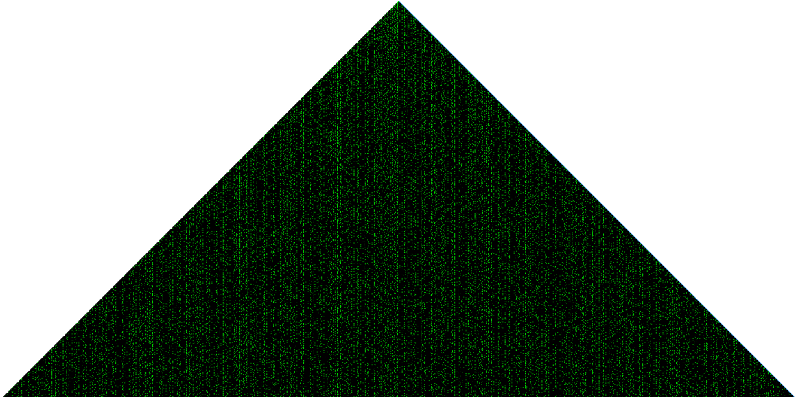
Fig 1: Pyramid of Primes up to 500,000
