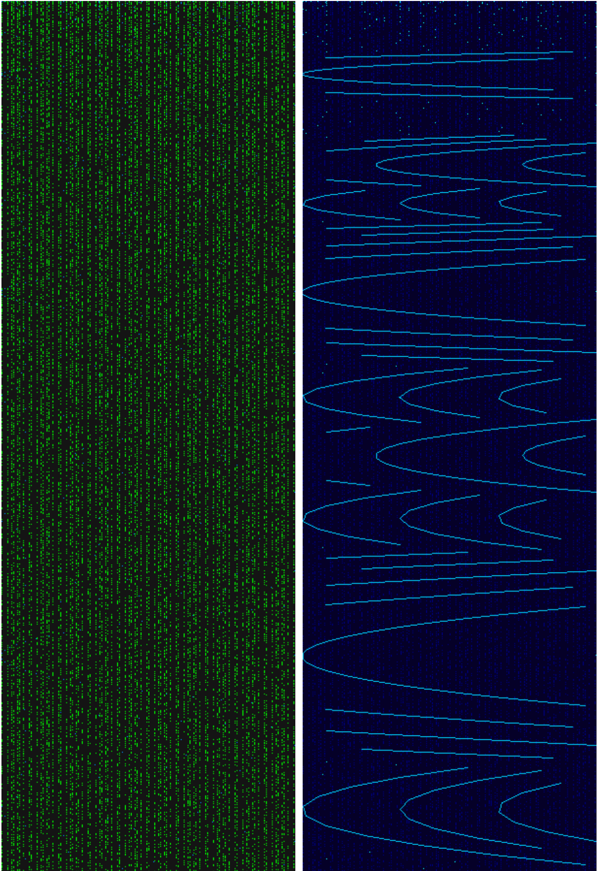
Fig 9: Block of Primes Mod 300 - Squares on right
