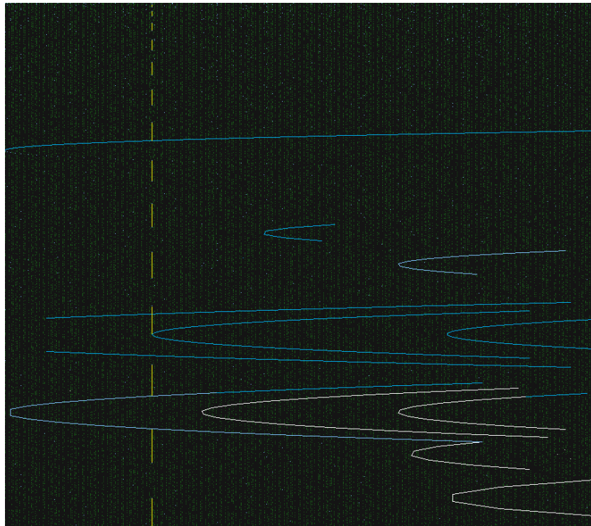
Fig 12: Block of Number Mod 1296 – Squares annotated
