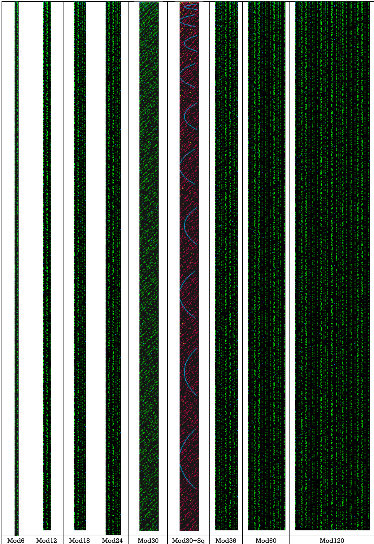
Fig 8: Blocks of Primes
