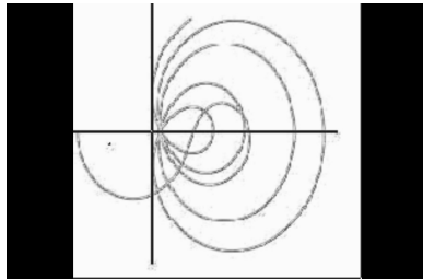
Figure 5: OUTPUT for \sigma = \frac{3}{5} with same axes definitions as that used in Figure 3.
