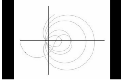
Figure 4: OUTPUT for \sigma = \frac{2}{5} with same axes definitions as that used in Figure 3.
