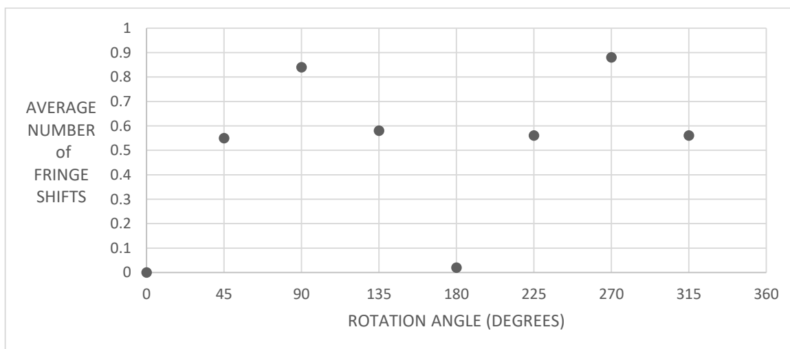
Chart 1 : Average fringe shift (in number of wavelengths) plotted against rotation angle.
