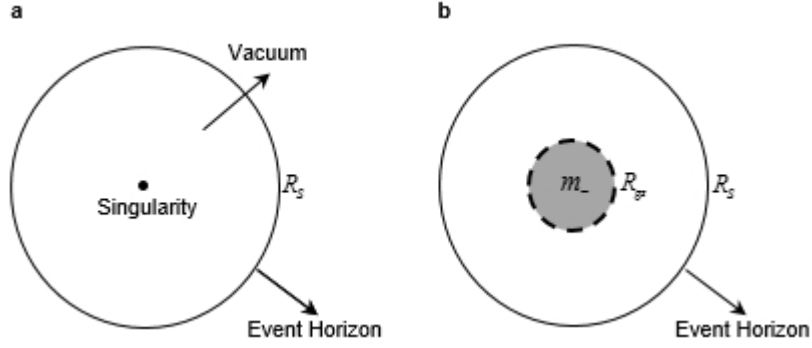
Figure 2: a.Existing Model. b.New Model. The area of within R_{gs} has gravitational self-energy of negative value, which is larger than mass energy of positive value. This area (within R_{gs} ) exercises anti-gravity on all particles entering this area, and accordingly prevents all masses from gathering to r=0 . Therefore the distribution of internal energy can't be reduced to at least radius R_{gs} = 0.3R_S .
