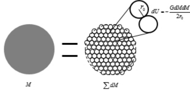
Figure 1: Since all mass M is a set of infinitesimal mass dM s and each dM is gravitational source, too, there exists gravitational potential energy among each of dM s. Generally, mass of an object measured from its outside corresponds to the value of dividing the total of all energy into c^2 .
