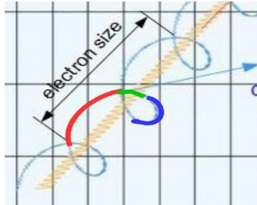
Fig.6. Electron red-shift from a moving reference frame
