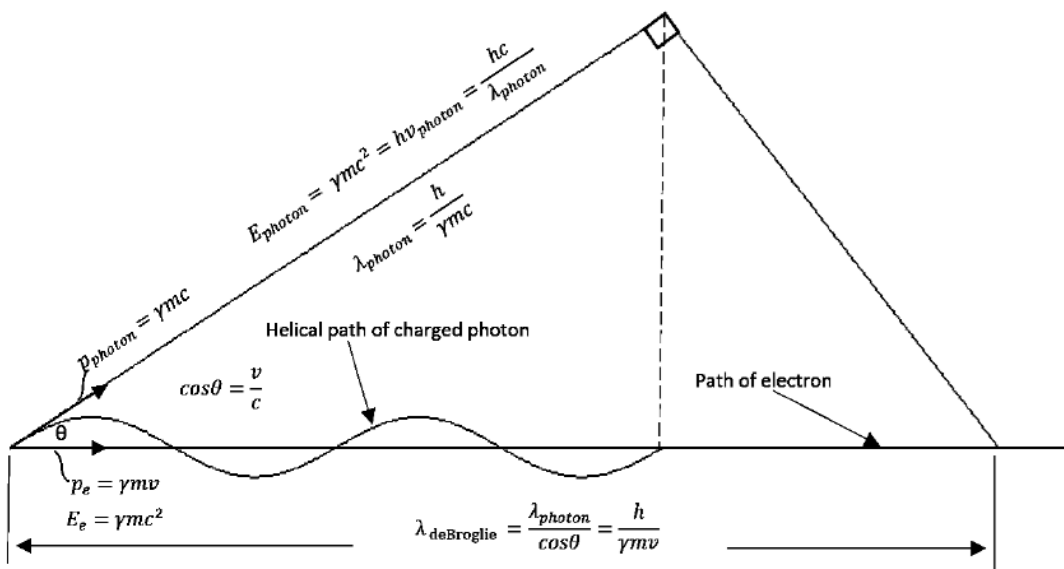
Figure 1. The electron’s de Broglie wavelength is generated from the spin ½ charged photon model of electron. The electron is moving to the right with speed v . The charged photon modeling the electron is moving helically to the right with speed c along its helical trajectory. The helical trajectory for one wavelength of the double-looping charged photon is mathematically unrolled to show the geometrical relations more clearly. Each wavelength of the double-looping charged photon along its helical trajectory generates the electron’s de Broglie wavelength along the helical axis of the charged photon. As the electron moves to the right with speed v , the de Broglie waves move to the right with speed v_{phase} = c^2 / v .
