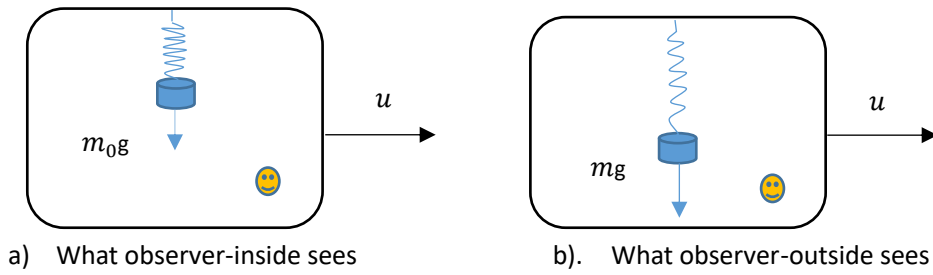
Fig.1. a spaceship is flying through a uniform gravitational field with the speed of u .
