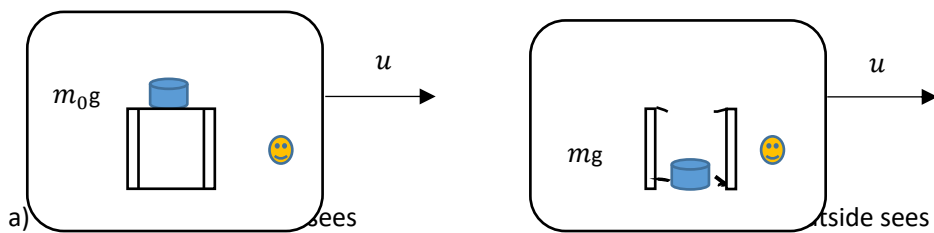
Fig.2. a spaceship is flying through a uniform gravitational field with the speed of u .
