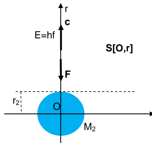
Fig.5 An energy quantum E moves away with radial direction from gravitational field generated by mass M_2 undergoing a small decrease of speed
