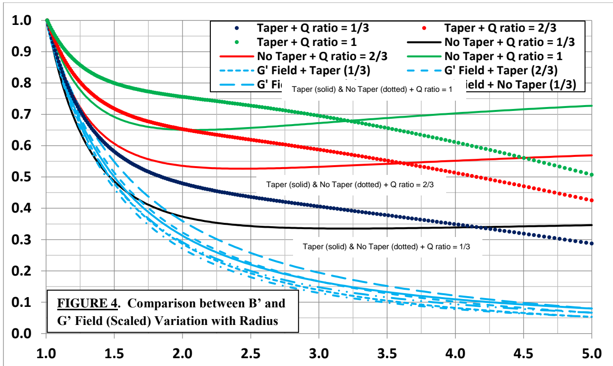
FIGURE 4. Comparison between B' and G' Field (Scaled) Variation with Radius
