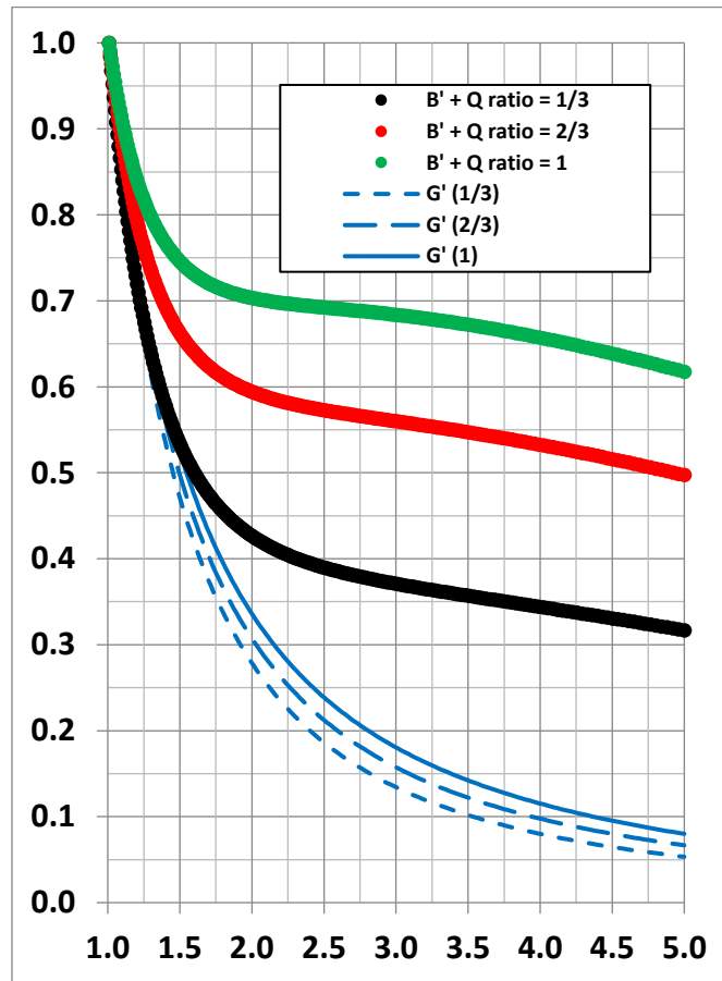
FIGURE 6. Scaled Average B' Fields between Taper and No Taper (with Halo of Globular Clusters)
