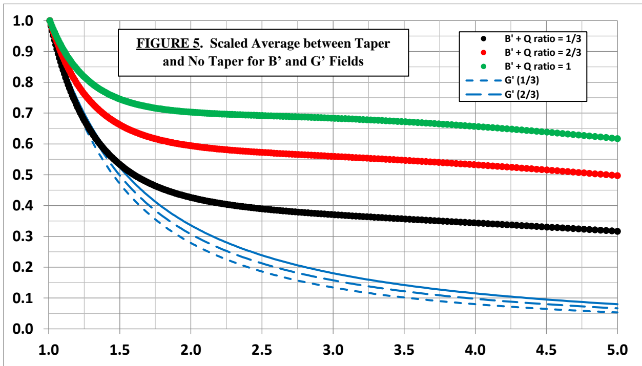
FIGURE 5. Scaled Average between Taper and No Taper for B' and G' Fields
