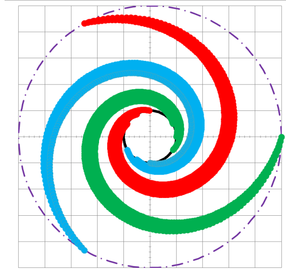
FIGURE 2. Representative Three-Armed, Logarithmic Spiral Galaxy
