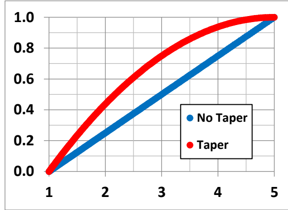
FIGURE 3. Variation in Disk Charge Fraction Based on Spiral Arm Tapering
