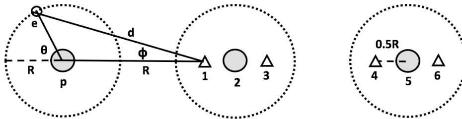
FIGURE 2. Geometric Arrangement of Three Hydrogen Atoms
