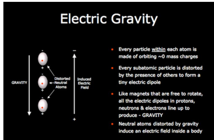
FIGURE 1. Explanation of Gravity by the Electric Universe Theory [1]
