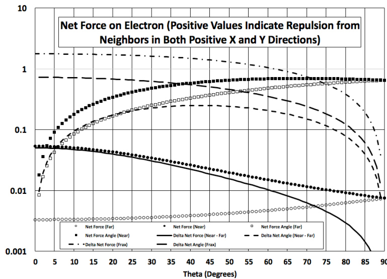
FIGURE 3. Net Force on Electron
