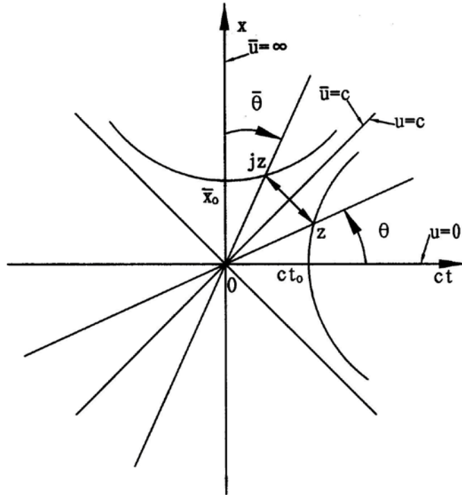
Fig. 1. NEW SPACE-TIME THEORY
