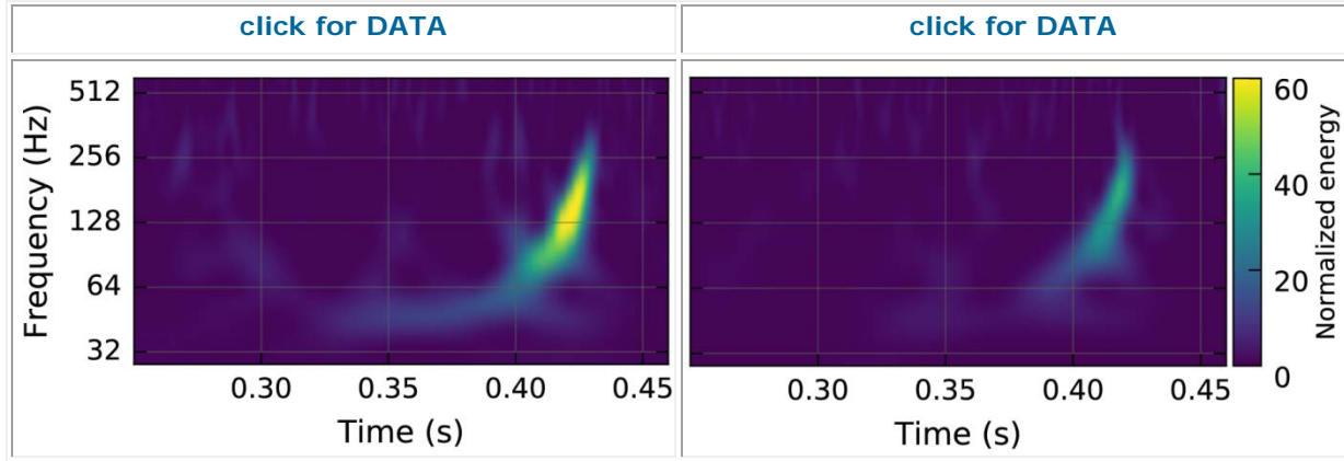
Fig.2. GW frequency scans from two LIGO detectors [1] . From the graphs it is abundantly clear that there is no frequency chirp down as the bodies approach their collision. Perhaps only a small region of a relatively stable frequency plateau that can be observed as is consistent with the graph for the new metric. This is clear evidence that there are no BHs only G-stars without EHs.
