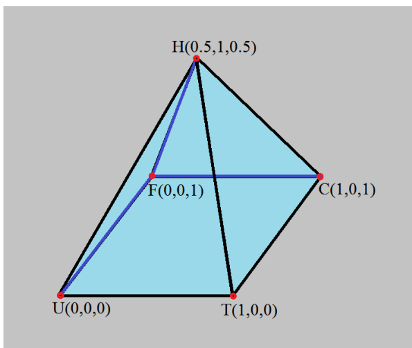
Fig. 6. Geometric representation of prototypes for features: truth, falsity, ignorance, contradiction and hesitation.
