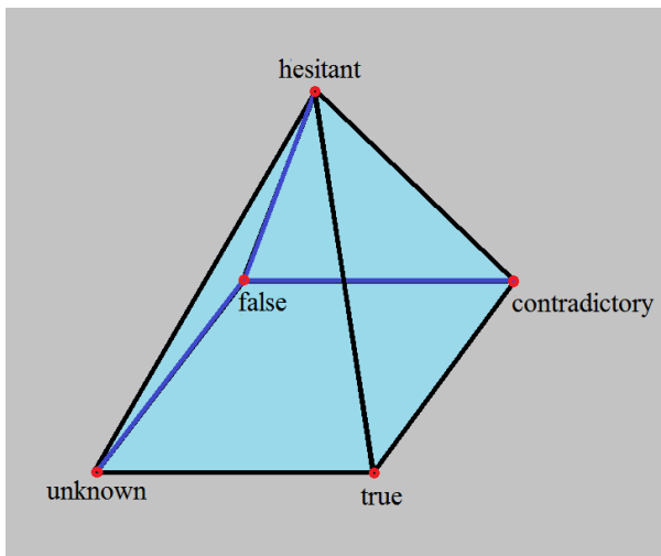
Fig. 5. The geometrical representation of the penta-valued space, based on true, false, unknown, contradictory and hesitant.
