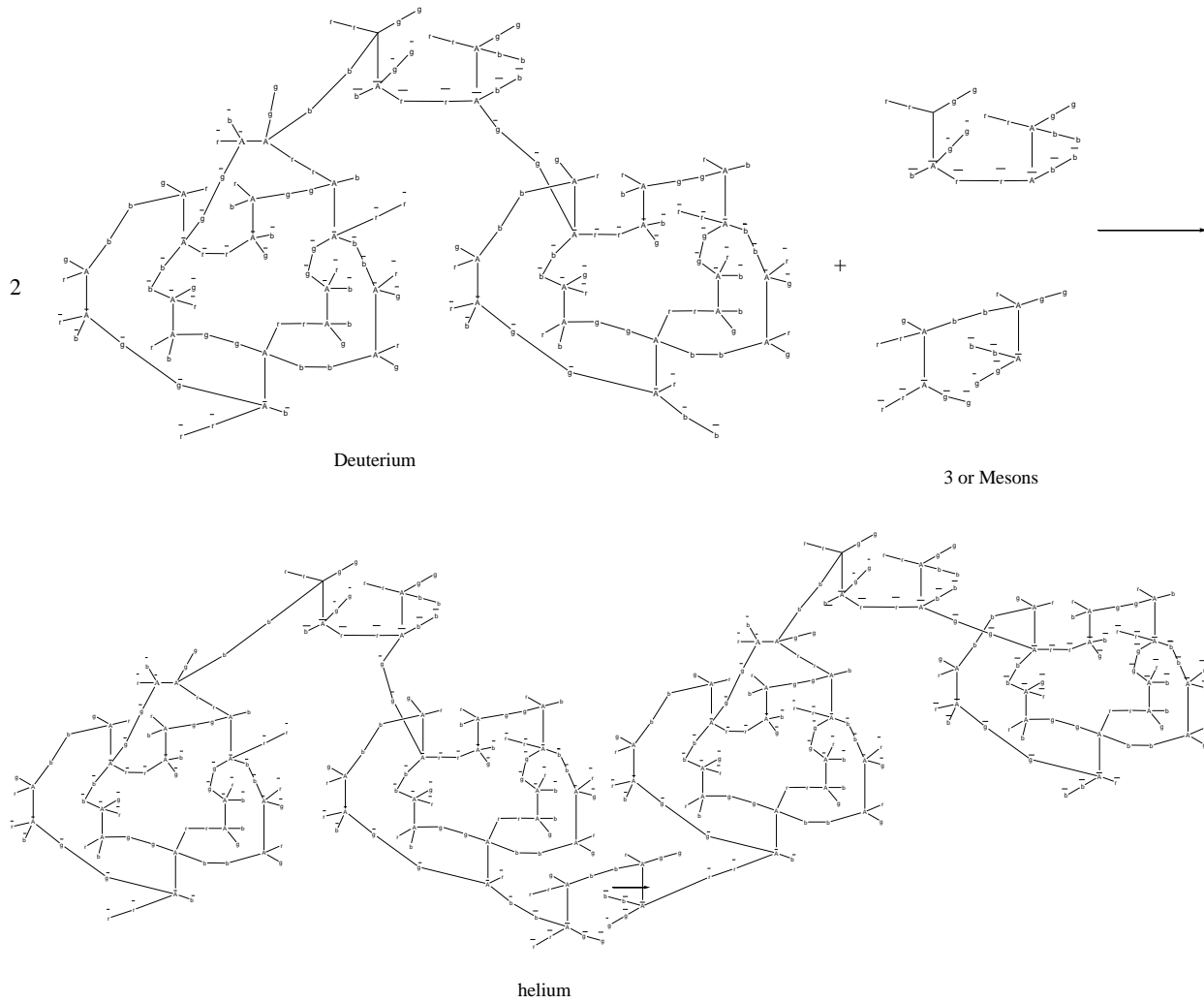
Figure 27. Fusion of Deuterium to Helium
