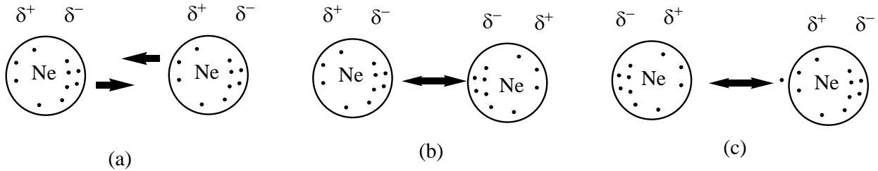
Figure 2. Distribution at Random of Instantaneous Dipoles of Neon: (a) attraction between partial negative and partial positive dipoles; (b) repulsion between partial negative and partial negative dipoles; (c) repulsion between partial positive and partial positive dipoles
