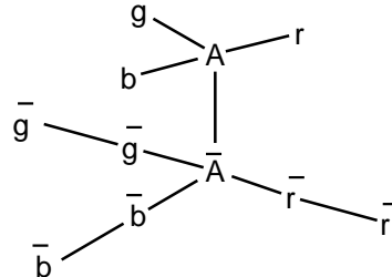
Structure 6. The Structure of Positron
