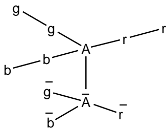
Structure 5. The Structure of Electron
