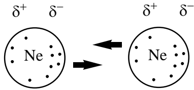
Figure 1. Attraction of Instantaneous Dipoles of Neon This process is at random and has equal chances to be:
