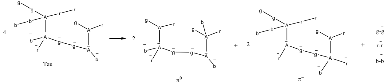
Scheme 9. Tau Decay
