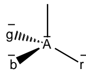
Structure 2. Anti Elementary Particles
