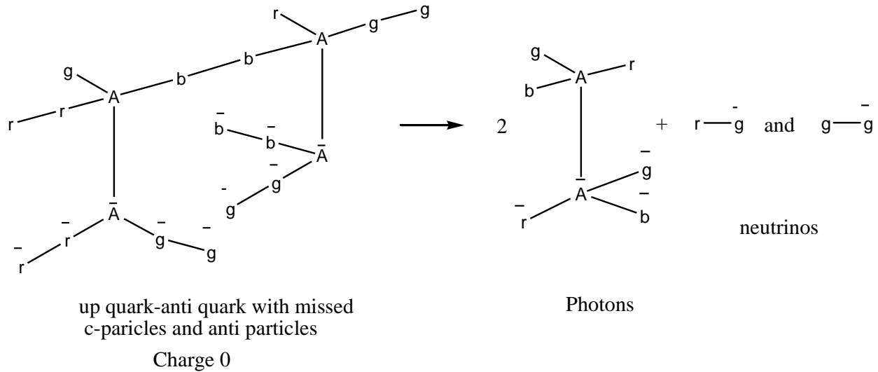
Scheme 12. Mesons without Charge Made from Up Quark and Up Antiquark with Missed c-particles and Anti Particles and Decay
