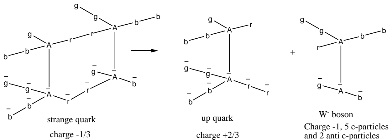
Scheme 2. Structure and Decay of Strange Quark
