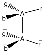
Structure 3. The Structure of Photon
