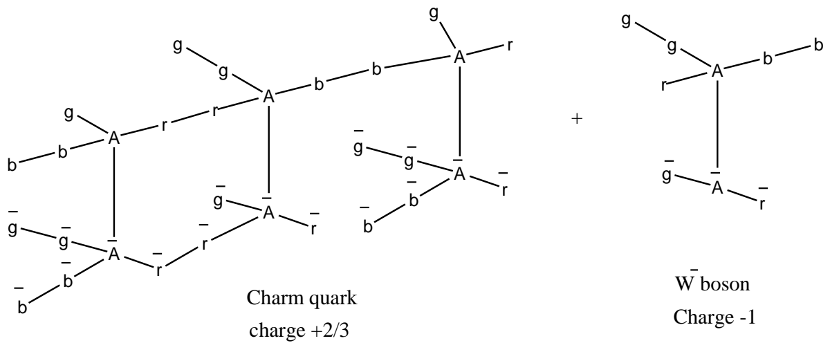
Scheme 4. Structure and Decay of Bottom Quark
