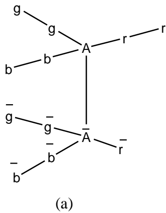
Structure 9. Structures of Down Quarks: (a); (b); and (c) are down quarks with different color charges
