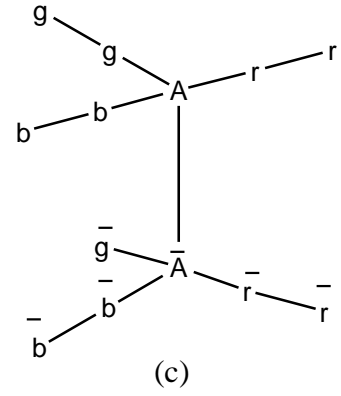
Structure 9. Structures of Down Quarks: (a); (b); and (c) are down quarks with different color charges
