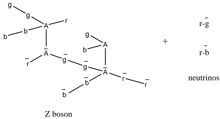
Scheme 6. High Energy Electron and Positron Annihilation
