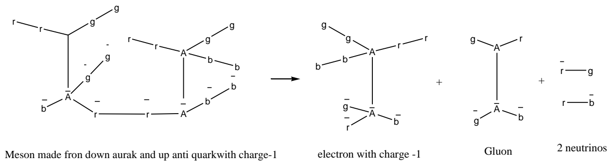
Scheme 13. Mesons with Charge Made from Down Quark and Anti Quark with Missed c-particles and Anti Particles and Decay.
