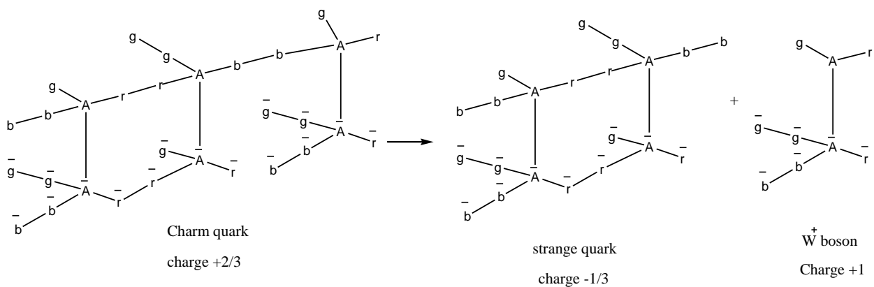
Scheme 3. Structure and Decay of Charm Quark
