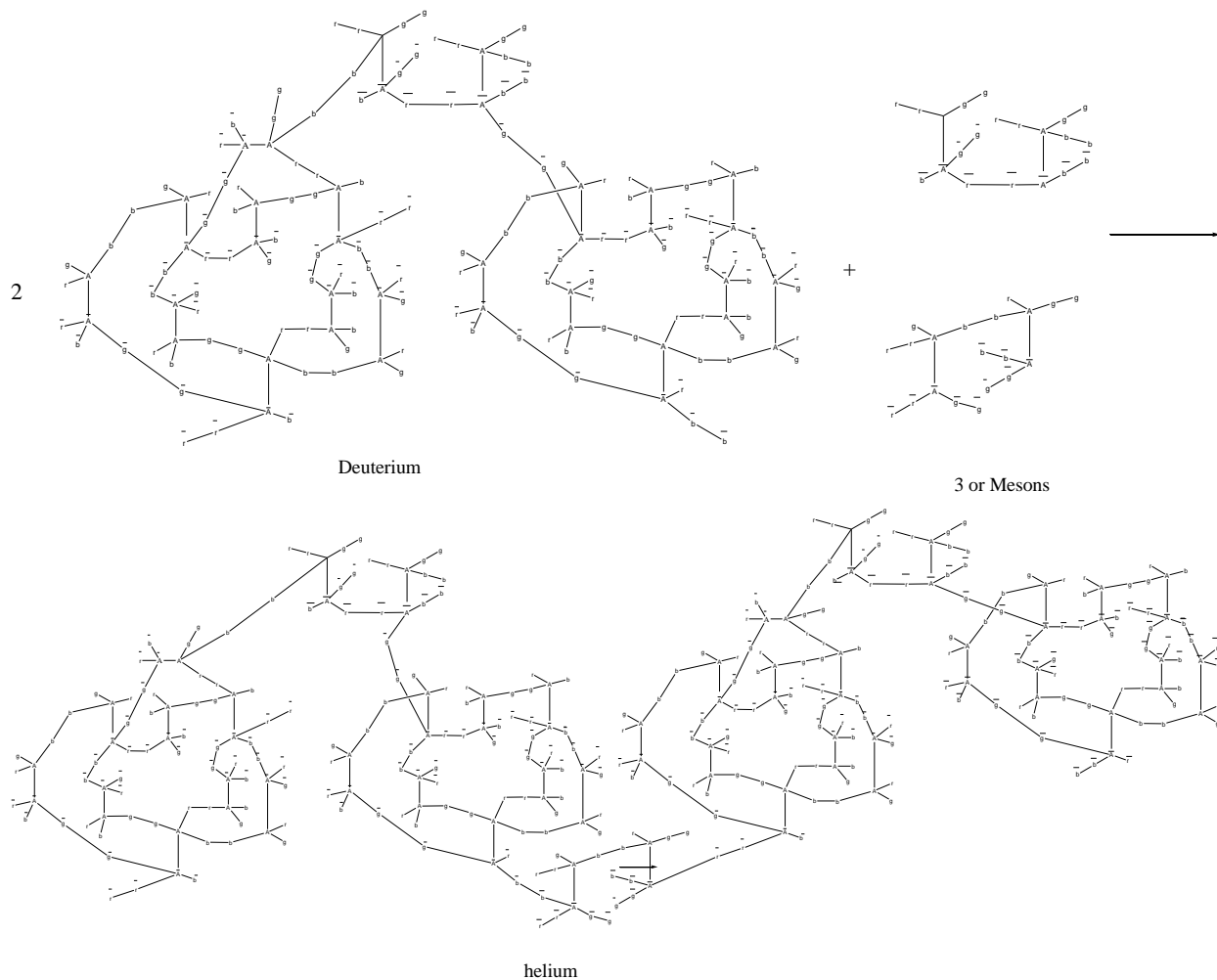
Scheme 14. Fusion of Deuterium to Helium
