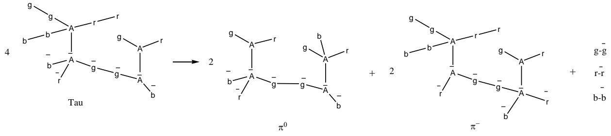
Scheme 9. Tau Decay
