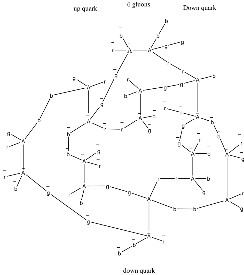
Structure 12. Structure of Neutron
