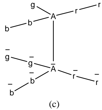
Structure 10. Structures of Down Antiquarks: (a); (b); and (c) are down antiquarks with different color charges
