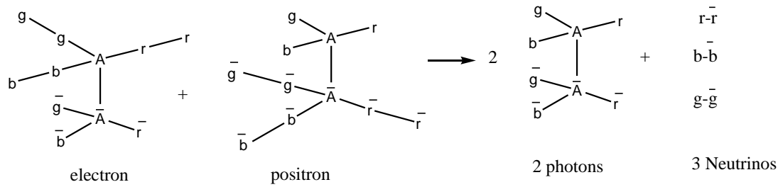
Scheme 10. Low Energy Electron and Positron Annihilation
