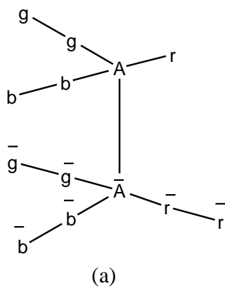
Structure 10. Structures of Down Antiquarks: (a); (b); and (c) are down antiquarks with different color charges
