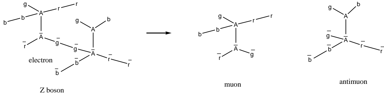
Scheme 7. Structure and Decay of Z Boson
