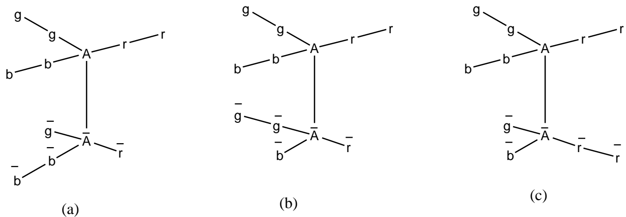
Structure 8. Structures of Up Antiquarks: (a); (b); and (c) are antiquarks with different color charges
