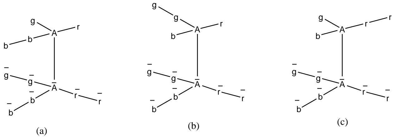
Structure 7. Structures of Up Quarks: (a); (b); and (c) are quarks with different color charges
