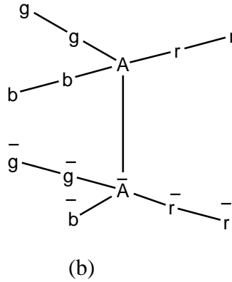
Structure 9. Structures of Down Quarks: (a); (b); and (c) are down quarks with different color charges
