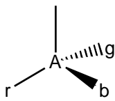
Structure 1. Elementary Particles
