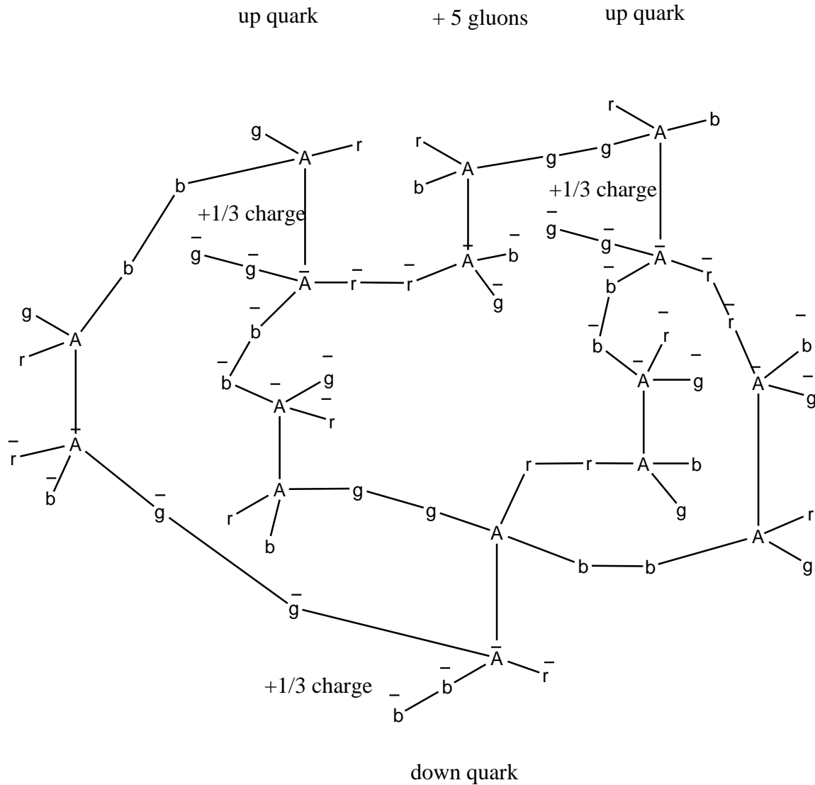
Structure 11. Structure of Proton( charge +1, spin 1/2)
