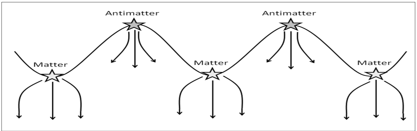
Figure 6 Illustration of how an SG anomaly centered by gravitational valley (positive curvature) and surrounded by large side-lobes can also produce multiple images. Arrows indicate how light paths will be altered by the curvature of space, and how light from the same object can reach us by multiple paths.
