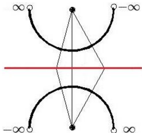
Fig. 12.1, adapted from Eric Schechter Fig. 12.2, sphere \leftrightarrow saddle transitions
