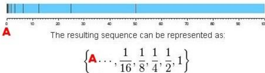
Fig. 20, adapted from Wikipedia ; compare with Fig. 11
