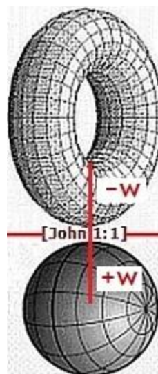
Fig. 12.1, adapted from Eric Schechter Fig. 12.2, sphere \leftrightarrow saddle transitions
