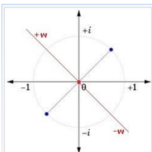
The two square roots of i in the complex plane (Wikipedia)
