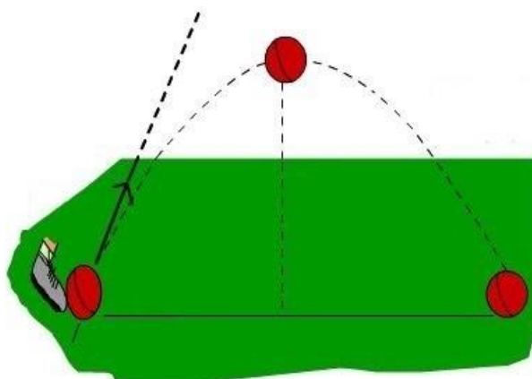
Fig. 1. Projective motion, adapted from Physics Tutorials
