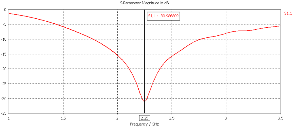
Fig. 5. The simulated return loss for the proposed antenna with the human head model
