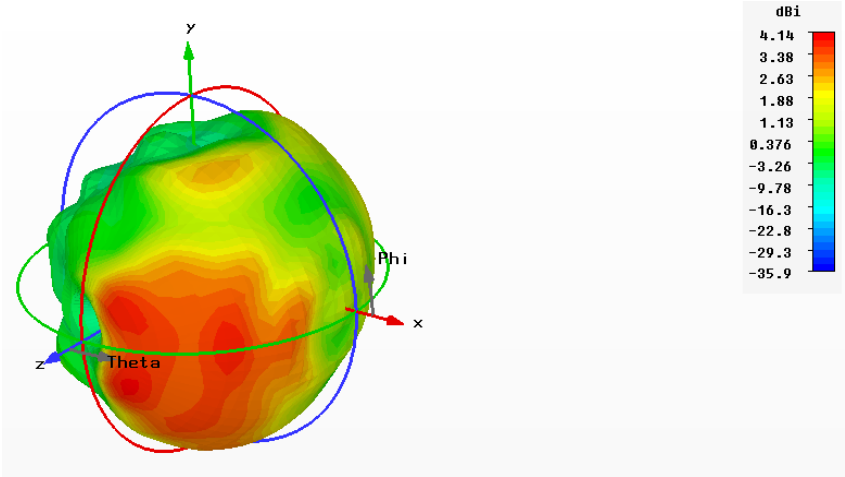
Fig. 6.. The radiation pattern for the proposed antenna with the human head model
