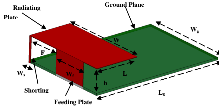
Fig. 1. The Geometry of the studied PIFA antenna
