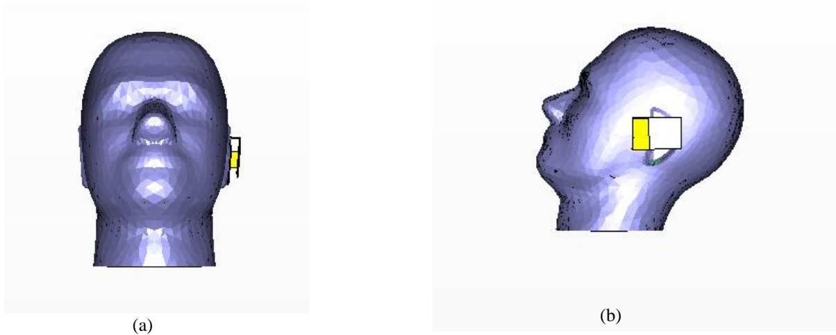
Fig. 4. The PIFA antenna next to the model of the human head
