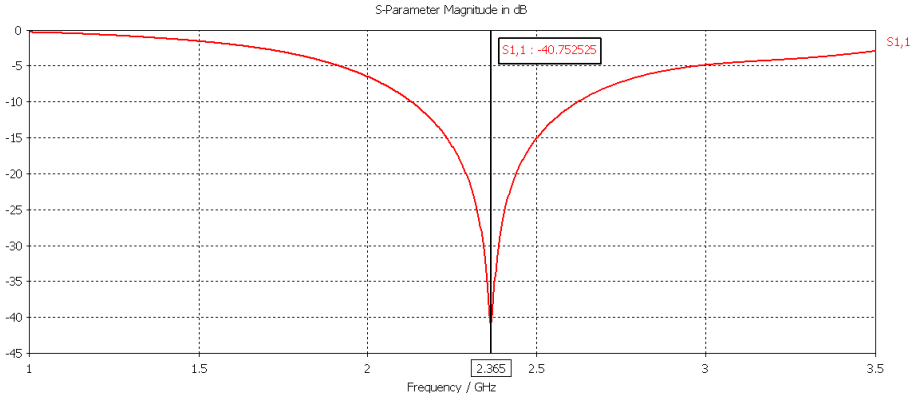
Fig. 2. The simulated return loss for the proposed antenna without human head
