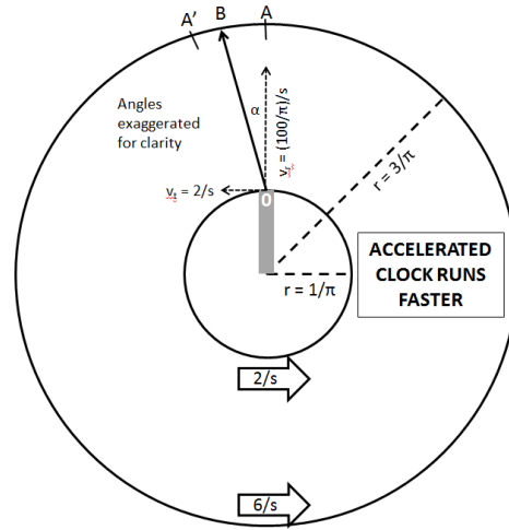
FIGURE 2. Case 2 – Carousel Rotating at Constant Speed with Gun Mounted on Inner Rim – Directional Acceleration Only
