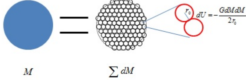
Figure 6: Since all mass M is a set of differential mass dM s and each dM is gravitational source, too, there exists gravitational potential energy among each of dM s. Generally, gravitational potential energy by differential mass that consists of an object itself is reflected on the mass of the object itself. Mass of an object measured from its outside corresponds to the value of dividing the total of all energy into c^2 .
