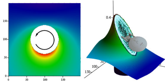
Figure-1, Space-time around a rotating mass-energy pressure field ( p ) and the resulting warp bubble
