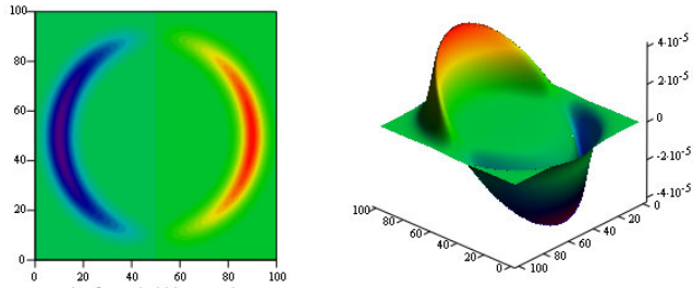
Figure-2, Exotic matter warp metric 4 top view and isometric view compared to superfluid results
