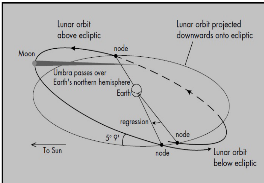
Fig. 1.5. The plane of the lunar orbit is tilted by just over 5^\circ with respect to the ecliptic, i.e. the Earth's orbit around the Sun. In addition, the line of the nodes (the plane intersection points where eclipses occur as Earth, Moon and Sun are in line) regresses clockwise by 19^\circ per year. This regression gradually shifts the two windows per year when eclipses can occur, earlier, by about 19 days per year. As shown in the diagram, when the nodes are at right angles to the Sun–Earth line, the Moon's umbra will sail way above (or below) the Earth at New Moon.
