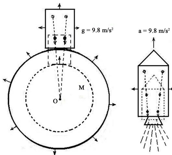
Figure 4. The full equality of expansion with the gravity.
