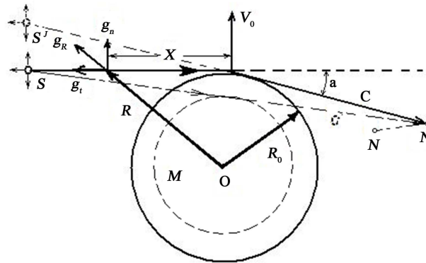
Figure 6. Light rays deviation near massive body. M, R_0 : massive body; S : light source; N : observer's location; C : light ray; a : deviation angle.
