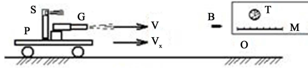
Figure 1. P: platform; O: observer; B: bullet; V: speed of bullet; V_x : speed of platform; G: the gun; S: the source of light signals; T, M: the clock & meter.
