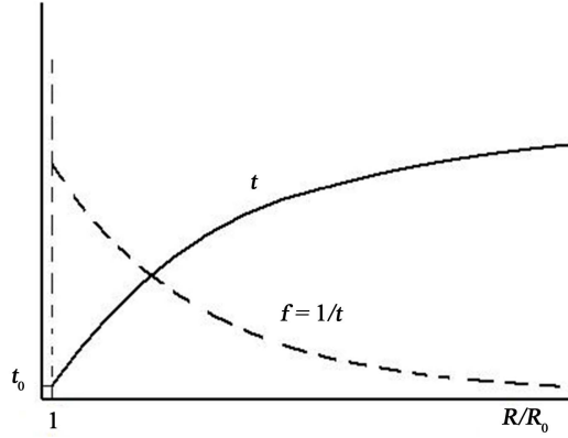
Figure 7. Time change with expansion.
