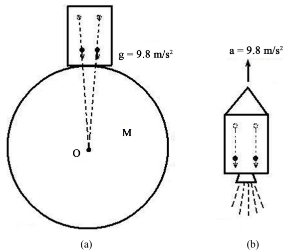
Figure 3. The difference of trajectories in free falling (a), and in the acceleration (b).
