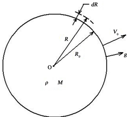
Figure 5. The expansion of material body.
