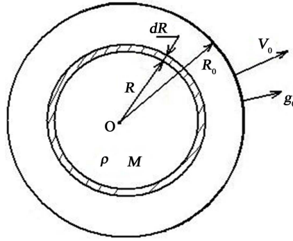
Figure 8. The energy of expansion.
