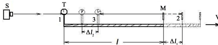
Figure 2. S: Light impulse source; T: Timer with photo scencore; l: The rod; M: The mirror. The task of experiment is to define light velocity in moving frame by direct measurements time of passage light pulses of the rod with the length— l . Timer—T starts work when light hits to it from left side of drawing (point 1) and it stops when light hits from right side (3), after reflection (point 2) from mirror: M, fixed in right end of the rod.
